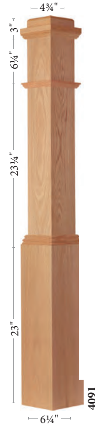
4091 Newel 6-1/4" x 55" POPLAR (78210) Mounting Block (78211)
