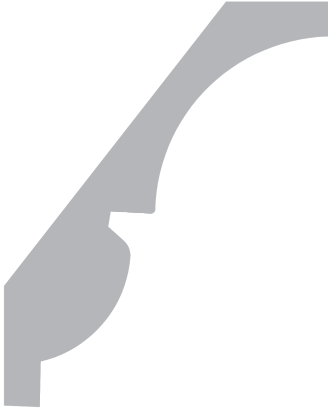
HL3532 1\frac{1}{16}'' \times 5\frac{3}{8}'' POPLAR (78827) Rise: 4" Run: 3\frac{1}{2}''
