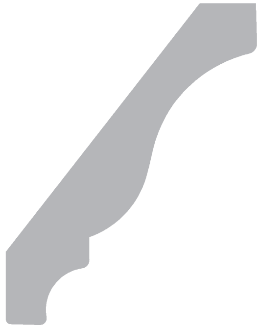
HL3425 3/4'' \times 41/4'' POPLAR (700367) FINGERJOINT POPLAR (171916) Rise: 33/8'' Run: 25/8''
